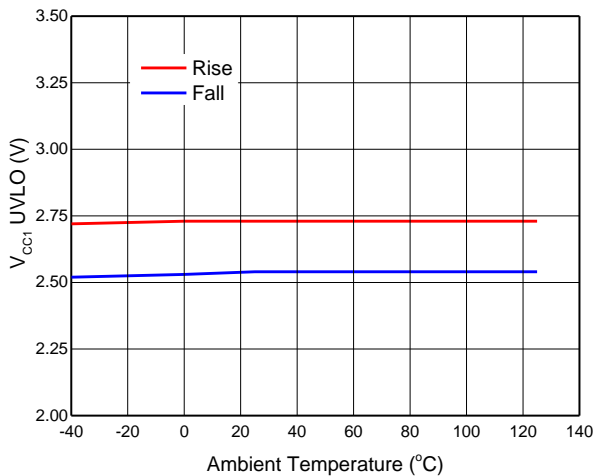
Figure 22. V CC1 UVLO vs Temperature
