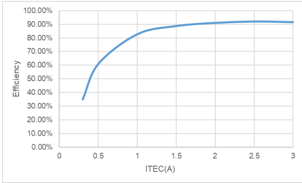
Figure 4. Efficiency vs. ITEC at V IN =5V with 1Ω in Cooling Mode
