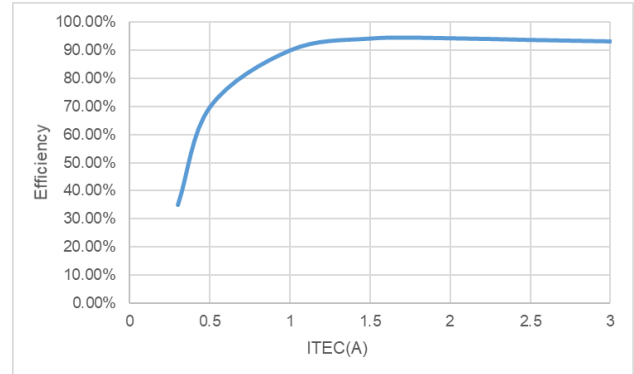
Figure 5. Efficiency vs. ITEC at V IN =5V with 1Ω in Heating Mode
