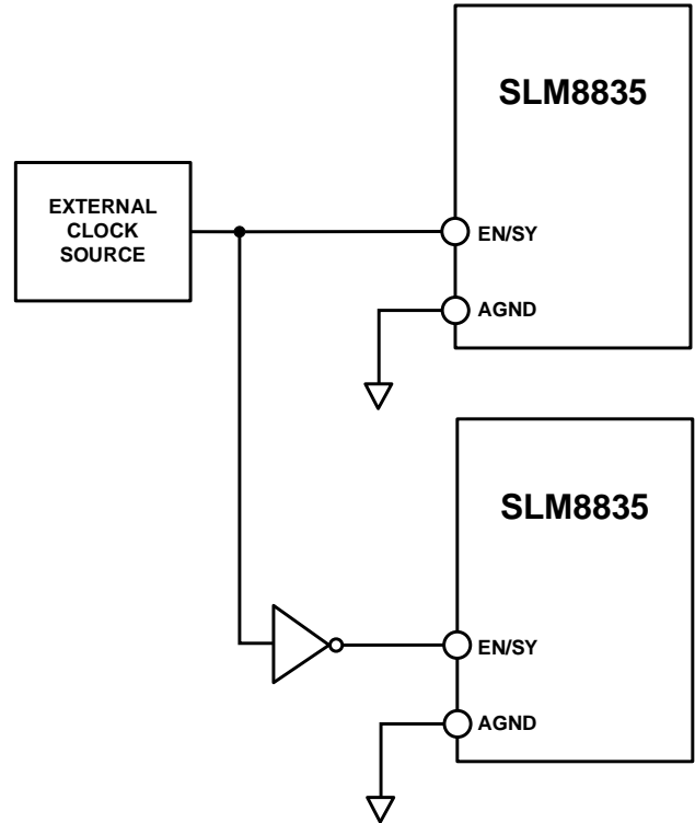
Figure 12. Multiple SLM8835 Devices Driven from a Master Clock
