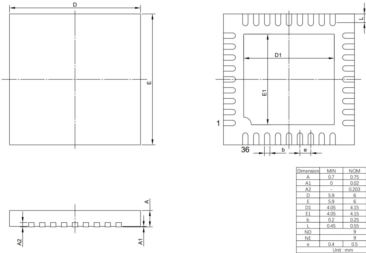
Figure 17. 36 Lead, 6mm x 6mm QFN Outline Dimensions
