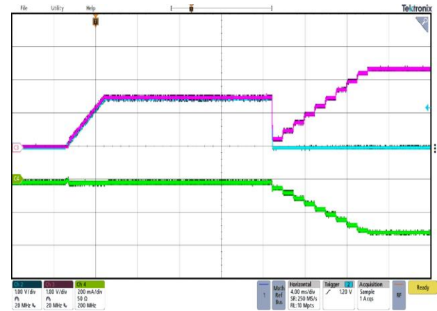
Figure 7. Soft Start into Heating Mode (V IN =3.3V with 5Ω load)
