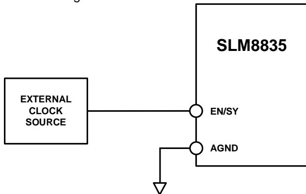
Figure 11. Synchronize to an External Clock
