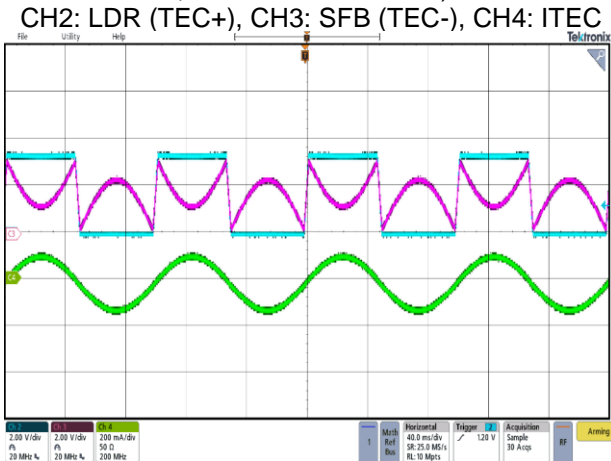
Figure 8. Cooling to Heating Transient CH2: LDR (TEC+), CH3: SFB (TEC-), CH4: ITEC
