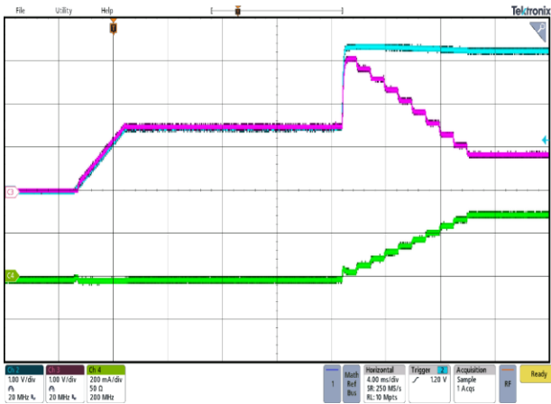
Figure 6. Soft Start into Cooling Mode (V IN =3.3V with 5Ω load)
