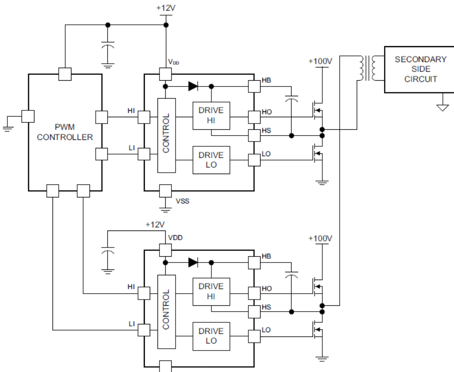
Figure 21. SLM27211 Typical Application Circuit in Full Bridge
